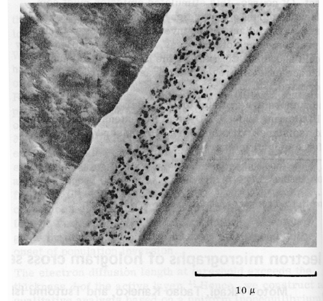
FIG. 5. Transmission-electron-microscope view of a cross section of a phase hologram A on Scientia 14C75 film.
