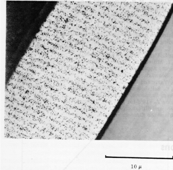
FIG. 3. Transmission-electron-microscope view of a cross section of a phase hologram A on Kodak 649F film.
