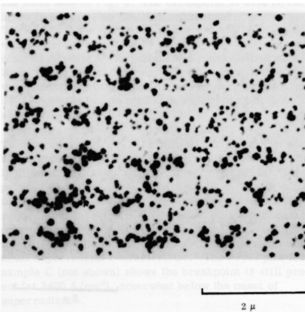
FIG. 4. Higher-magnification view of the same sample as in Fig. 3.
