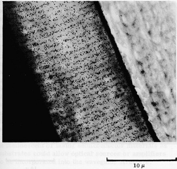
FIG. 1. Transmission-electron-microscope view of a cross section of an amplitude hologram A on Kodak 649F film.
