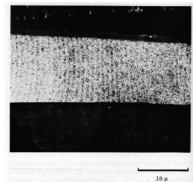
FIG. 6. Transmission-electron-microscope view of a cross section of an amplitude hologram B on Kodak 649F film.
