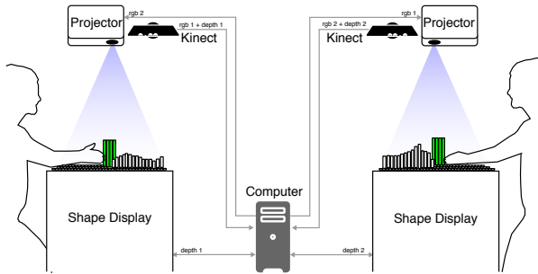
Figure 15. System diagram of connected workspaces with bidirectional shape capture and shape rendering.
